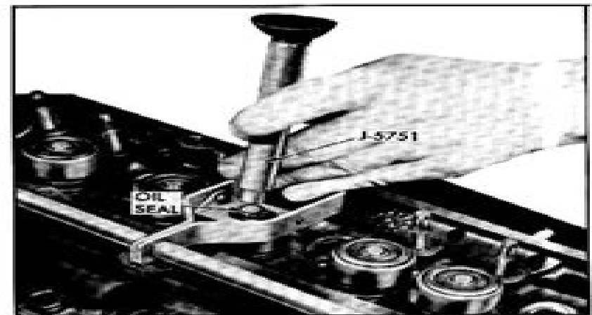
Fig. 6-48 Installing Valve Stem Seal
