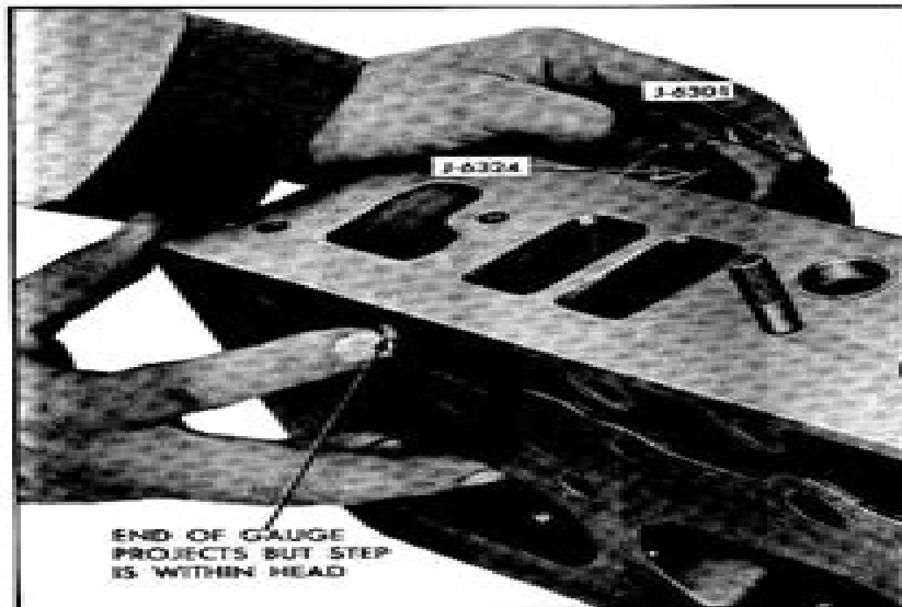
Fig. 6-46 Checking Length of Valve Stem
