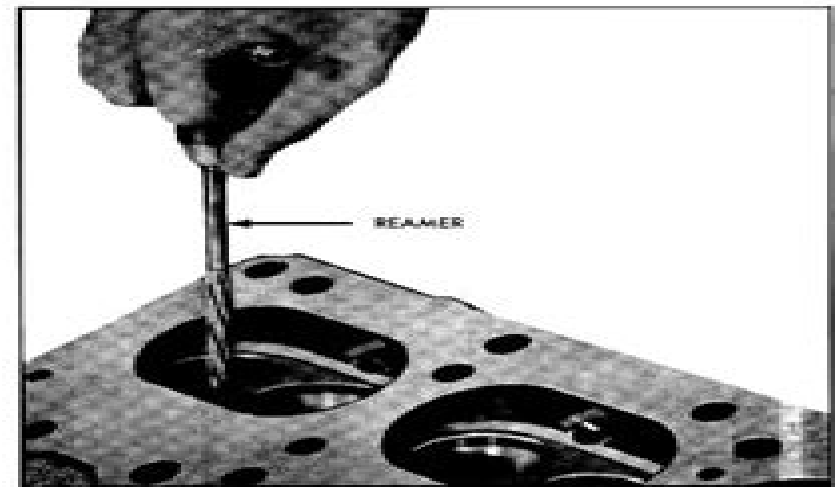
Fig. 6-47 Fitting Valve Stems to Guide
