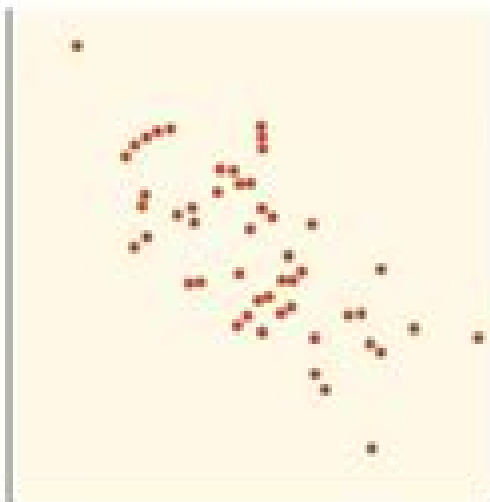
Correlation r = -0.7
