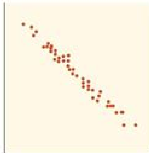
Correlation r = -0.99
