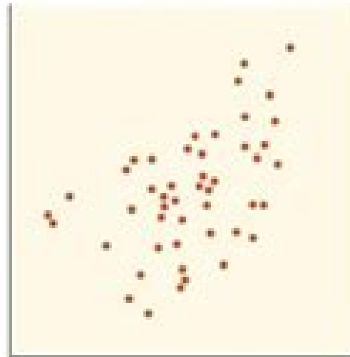
Correlation r = 0.5
