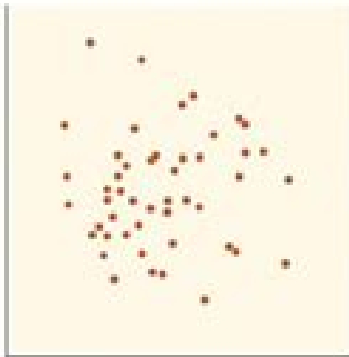
Correlation r = 0
