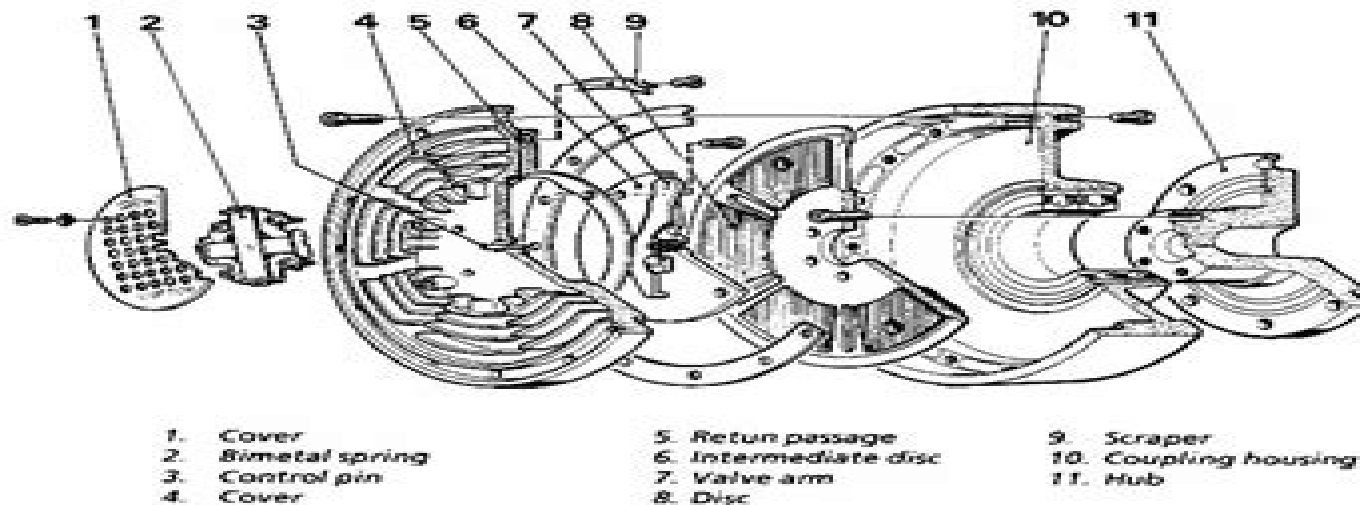
Coupling housing for temperature controlled fan
