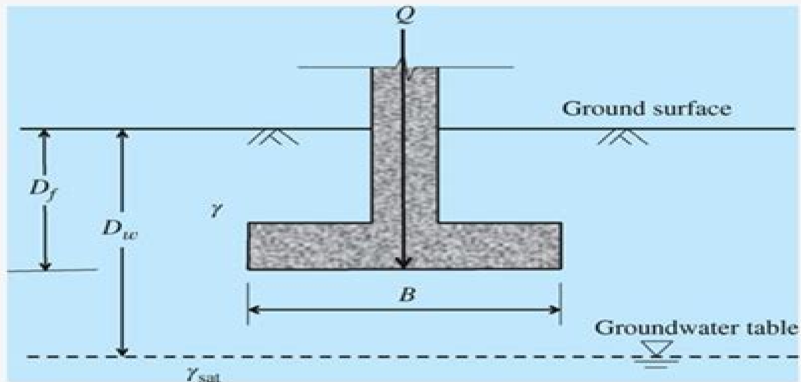
Fig. 3.9 Shallow foundation design sample problem.
