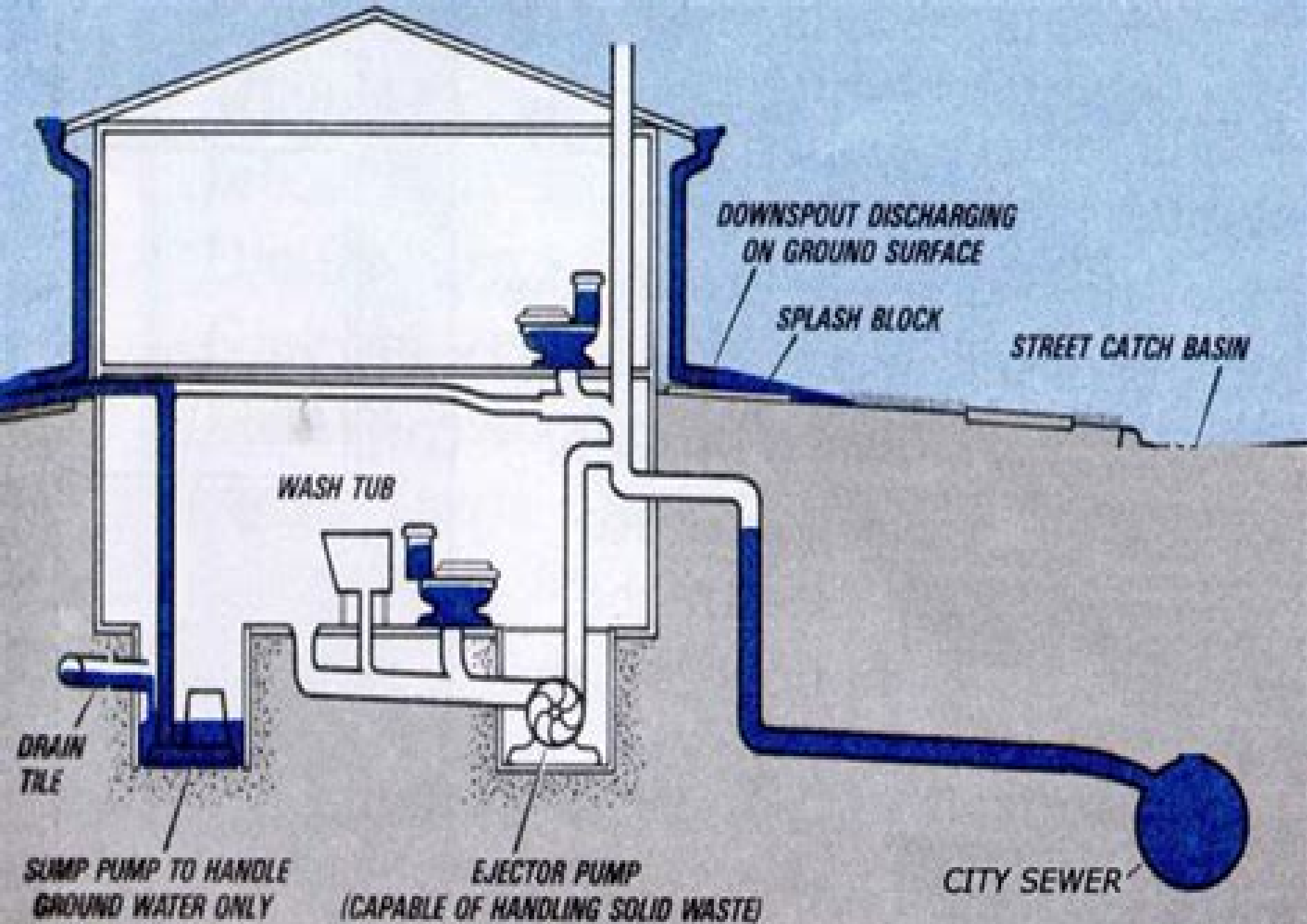
Flood Control Sewer Systems
