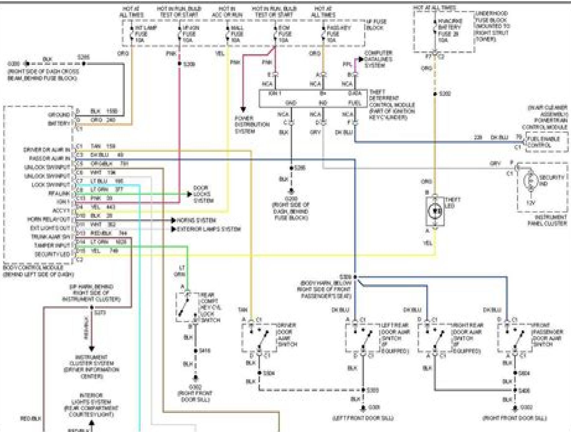
2002 Pontiac Grand Prix SE- Fig. 6: Anti-theft Circuit
