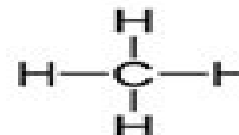
Methane molecule ( \text{CH}_4 )
