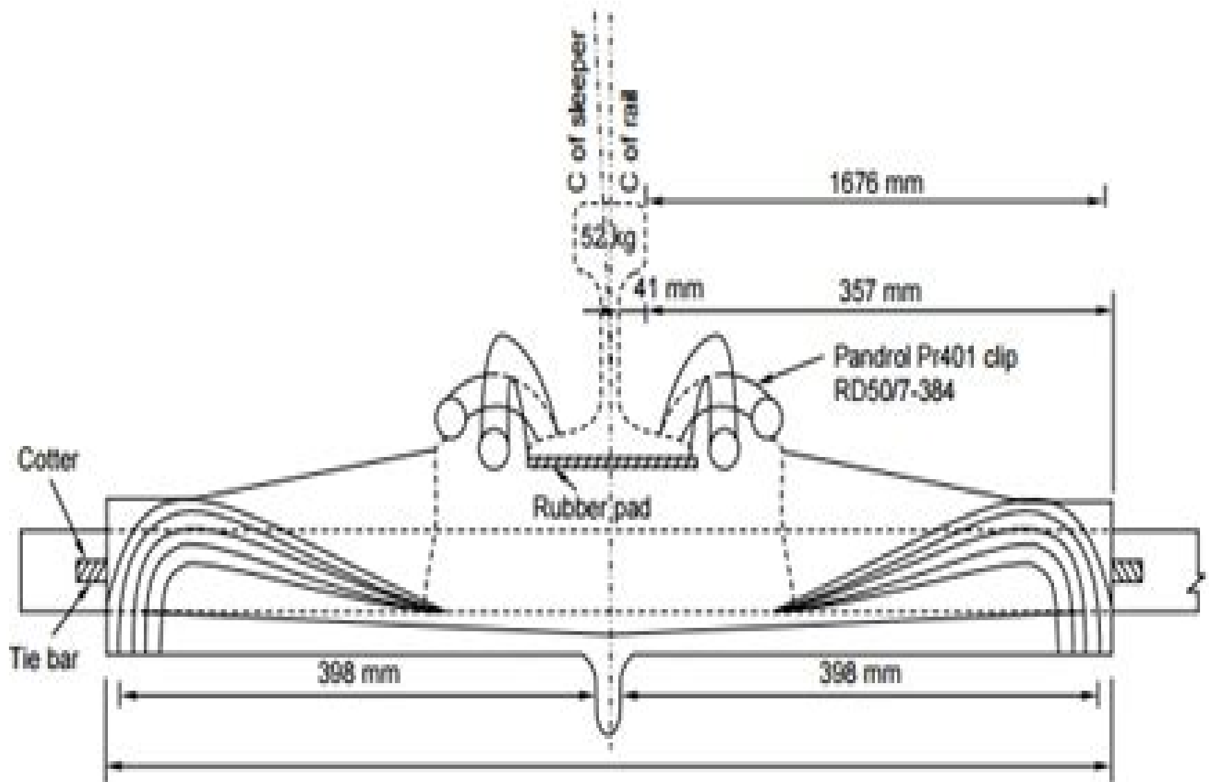
Fig. 10.16 Isometric view of Pandrol clip
