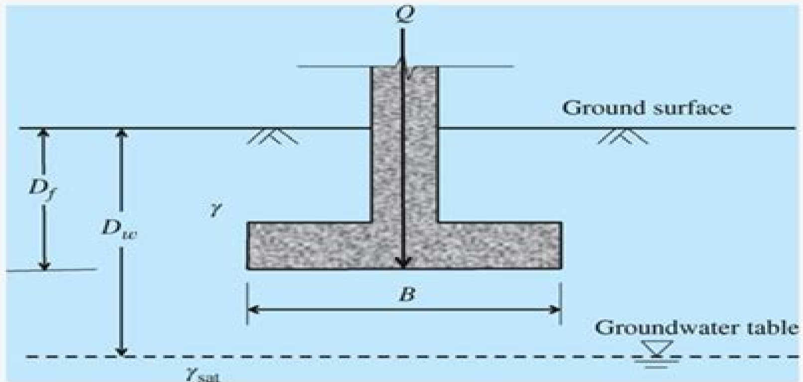
Fig. 3.9 Shallow foundation design sample problem.
