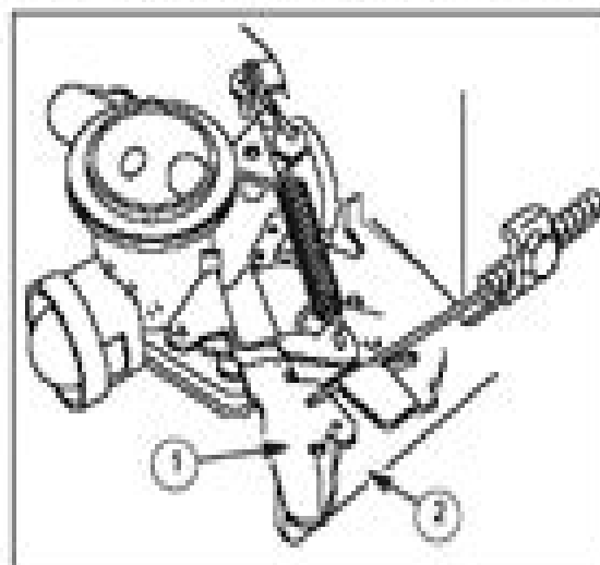
Fig. 96 - Remote Control
