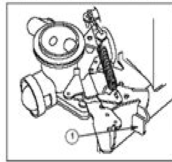
Fig. 97 - Fixed Adjustable
