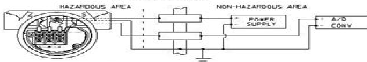
CIRCUIT DIAGRAM 4 TWO SINGLE CHANNEL BARRIERS (ONLY FOR USE WITH BARRIERS APPROVED IN THIS CONFIGURATION)
