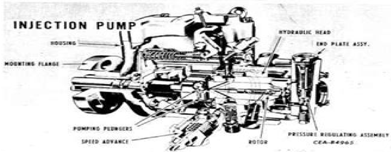
CUTAWAY VIEW OF MODEL DC INJECTION PUMP
