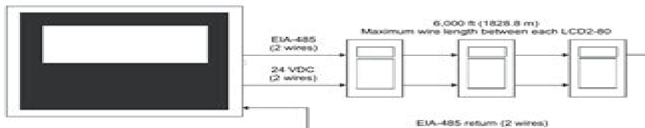
NFS-320, NFS2-640, NFS2-3030, or NCA-2 connecting to LCD2-80
