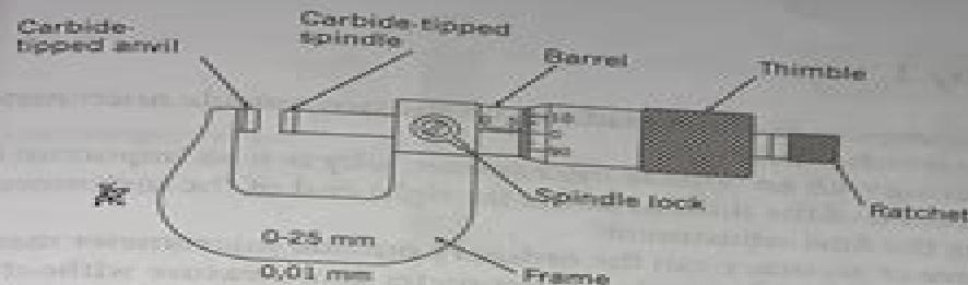
Figure 4.1: Outside micrometer
