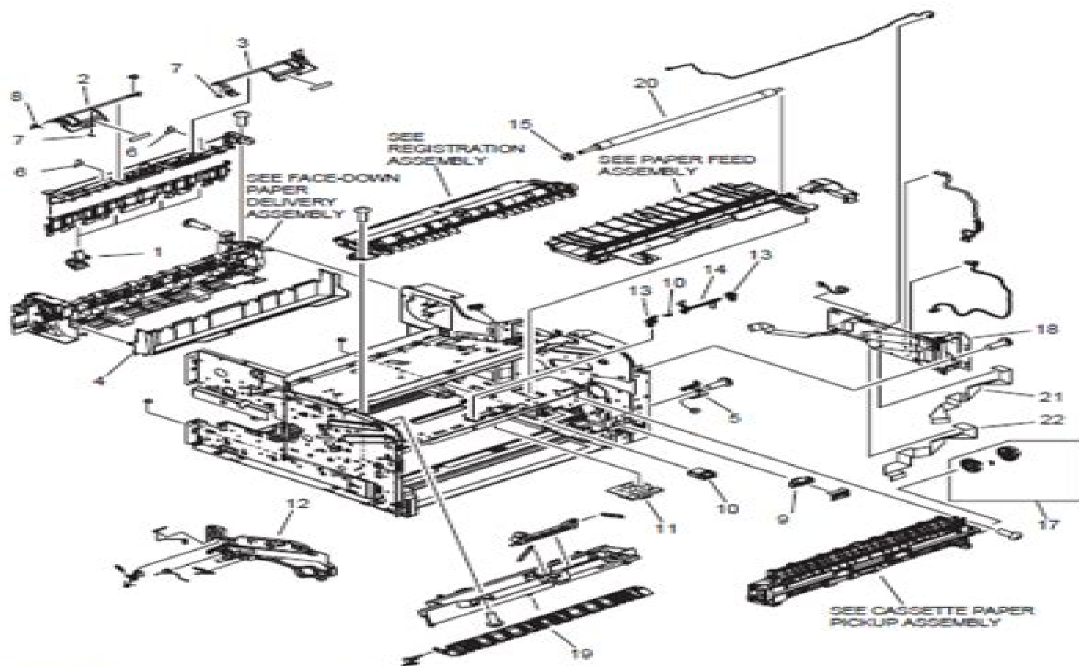
Figure 7-3 Internal components (1 of 3)
