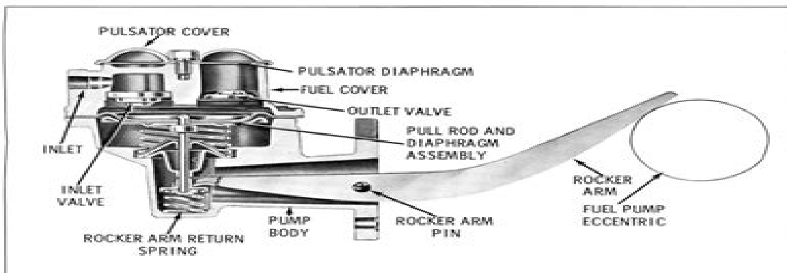
Fig. 3-133 Fuel Pump Assembly
