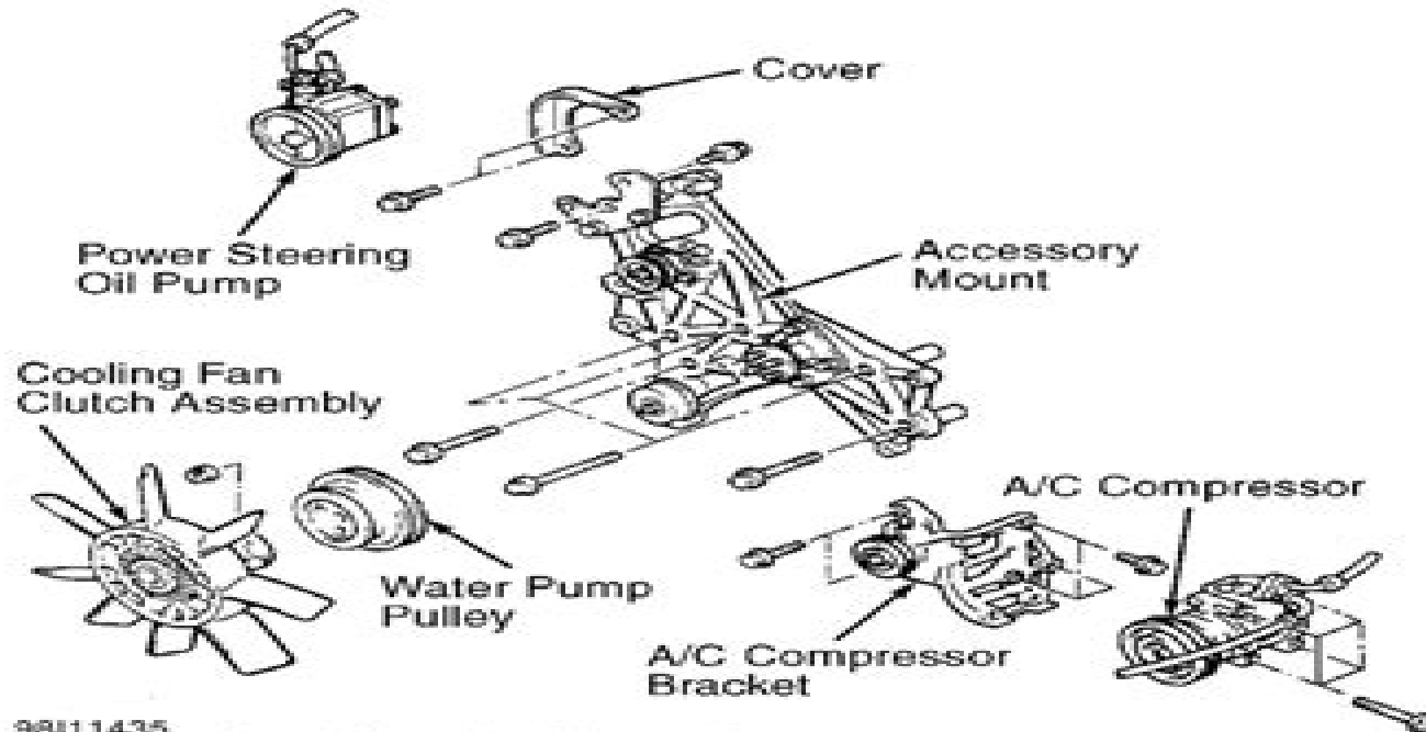
Fig. 1: Accessories & Mounting (Montero) Courtesy of Mitsubishi Motor Sales of America.
