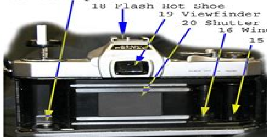
Manual SLR Film Camera Parts
