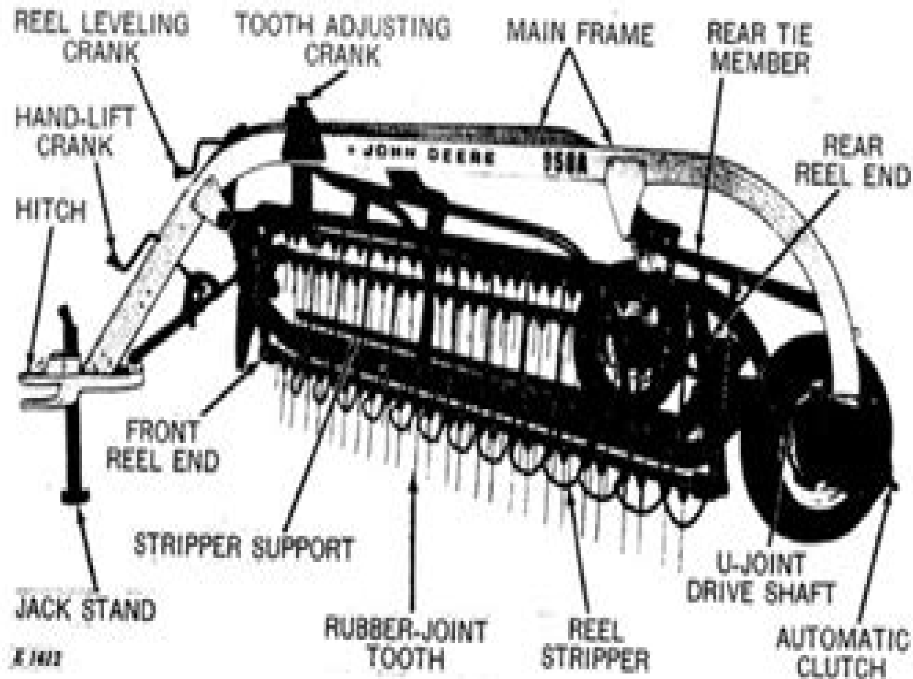
Left-Hand Side View of John Deere 858A Side-Delivery Rake
