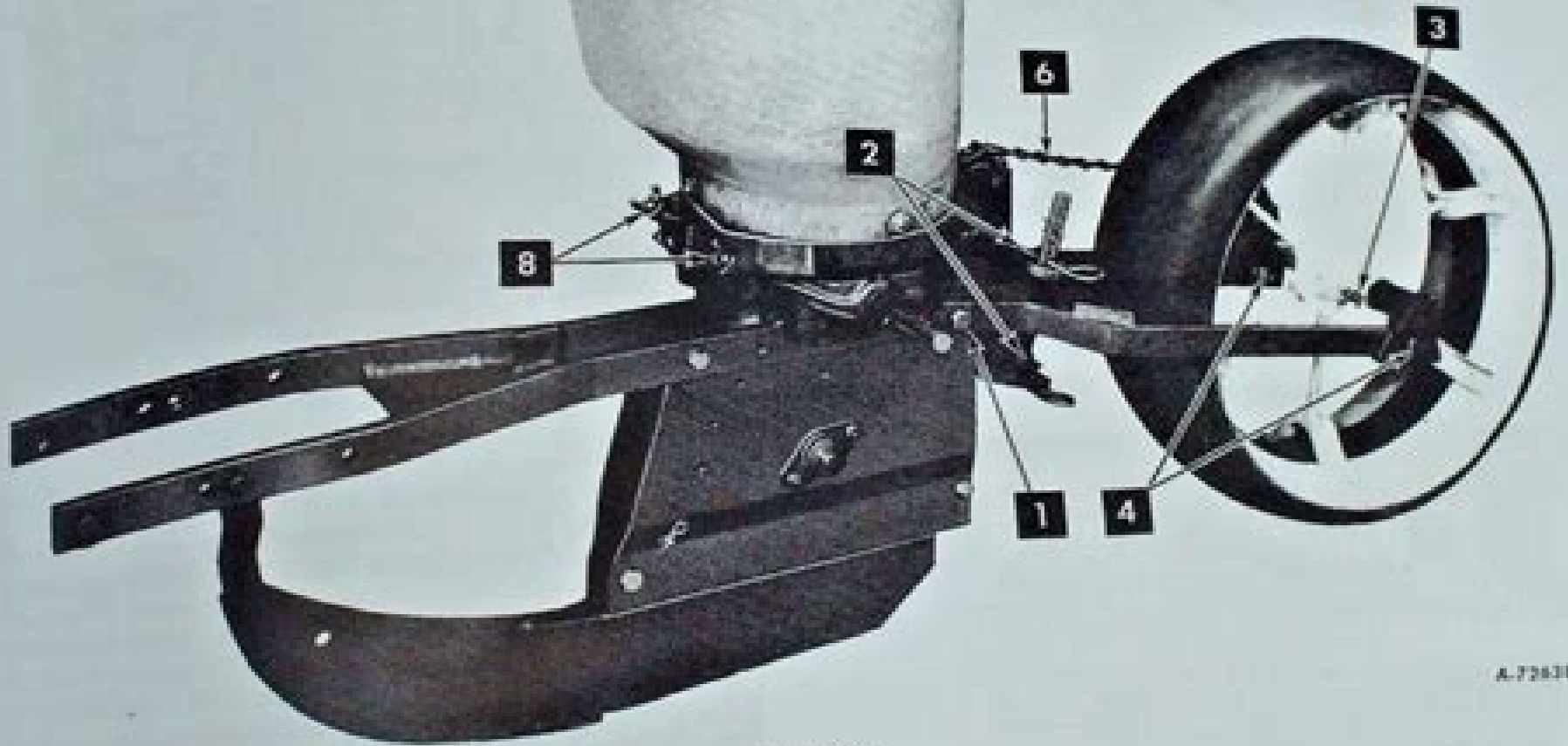
Illust. 35 186 Hill-Drop Planter 20" Press Wheel (regular) illustrated. (The rubber overtire shown must be obtained "special.")
