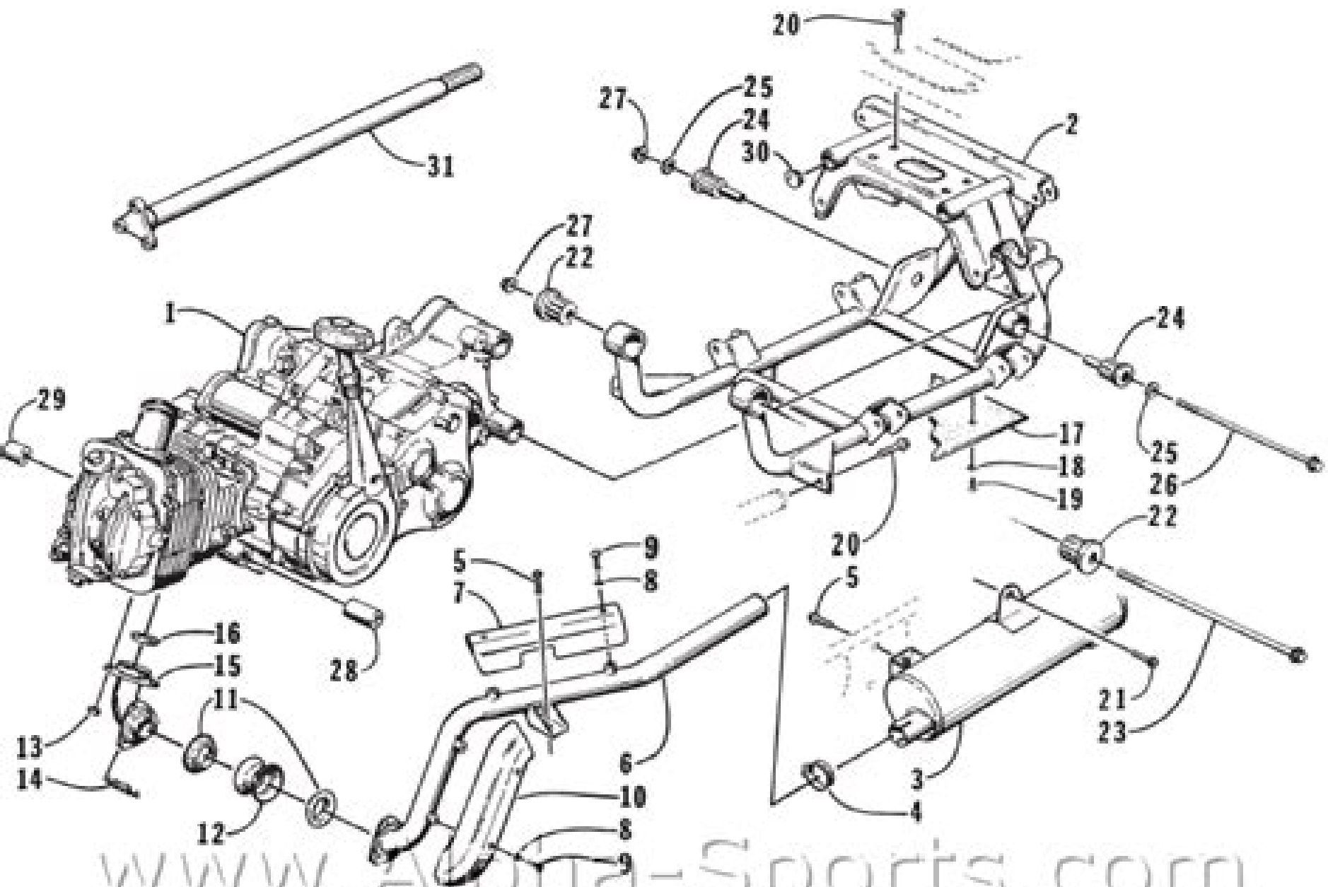
ENGINE AND RELATED PARTS
