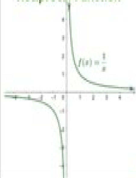
Reciprocal Function
