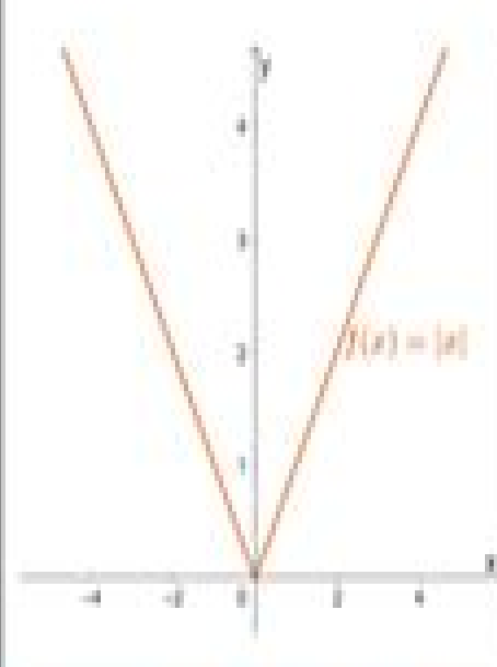
Absolute Function
