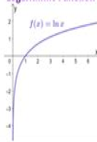
Logarithmic Function
