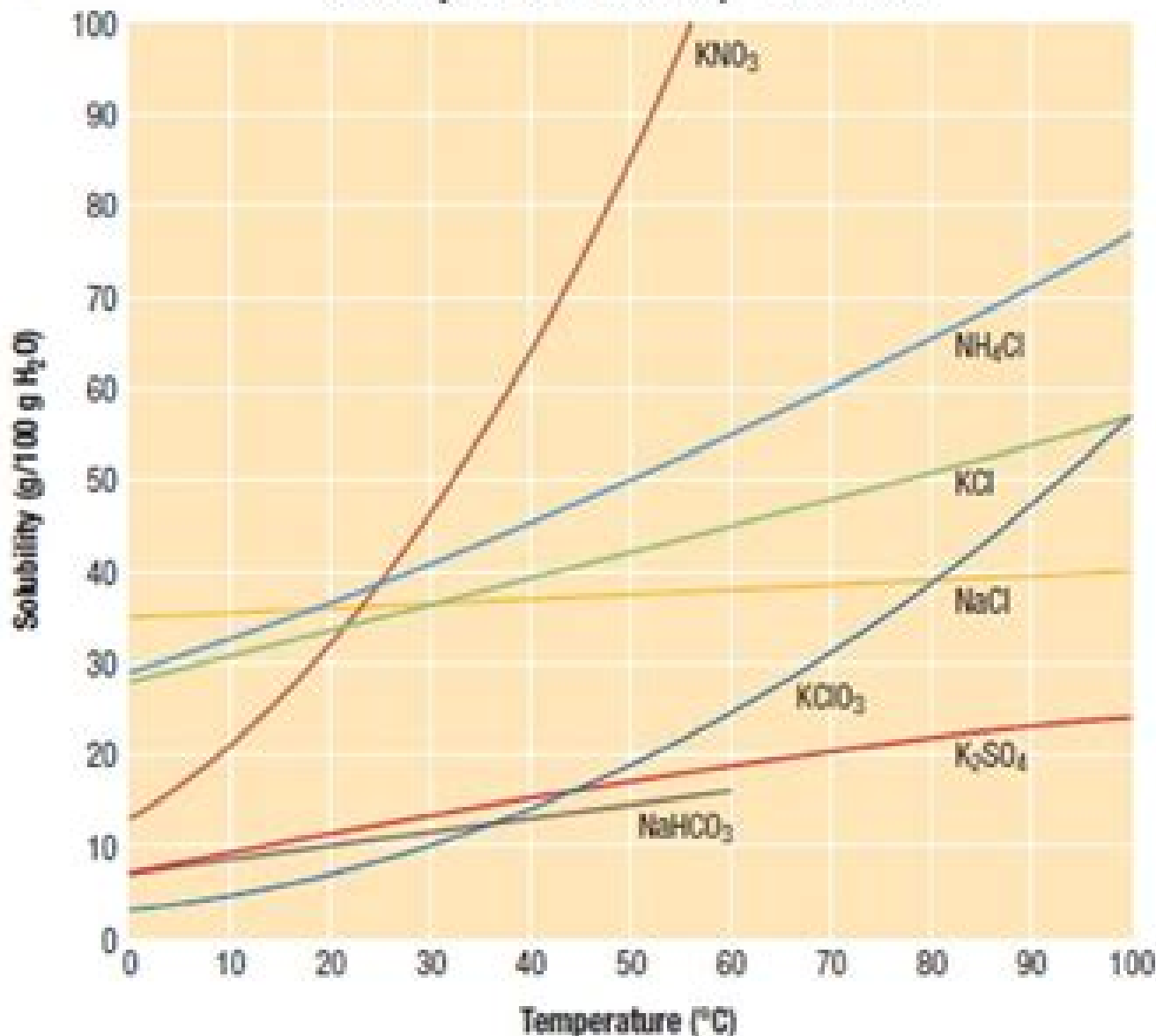
Solubility Curves of Ionic Compounds in Water
