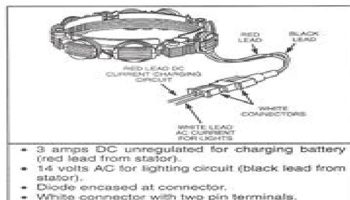
Fig. 2 - Dual Circuit Stator
