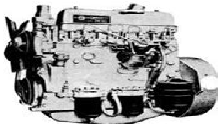
Figure 2 — GD-193 Diesel
