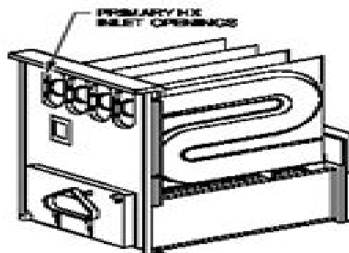
Fig. 6—Cleaning Inlet Openings of Primary Heat Exchanger
