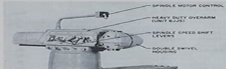
Figure 4A Style 1C Toolmaster Milling Machine with Heavy Duty Overarm and Double Swivel (Intermediate) Housing
