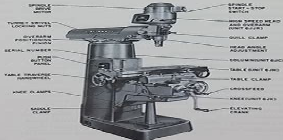
Figure 4B Style 1B Toolmaster Milling Machine with Power Feed to Quill, Manual Feed to Saddle and Table
