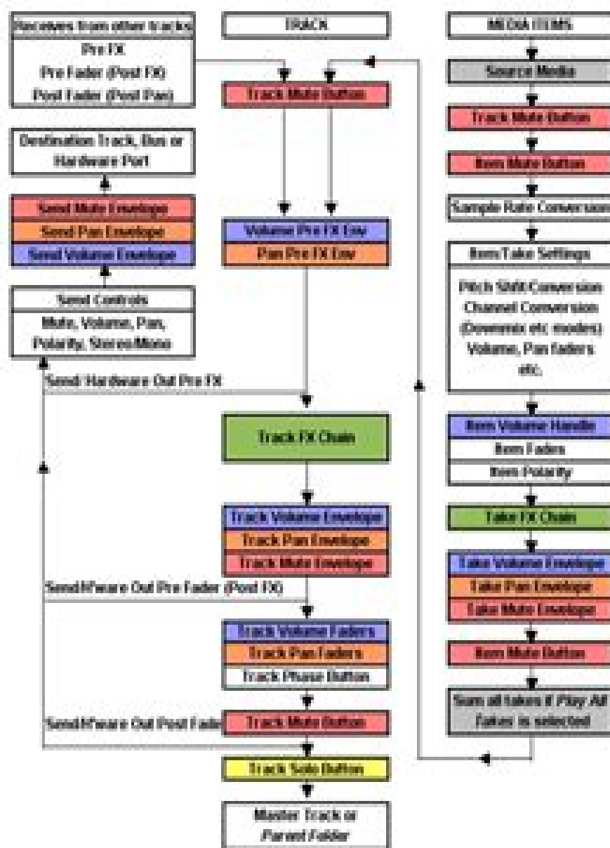
REAPER Audio Playback Signal Flow - Top Level Track or Child Track
