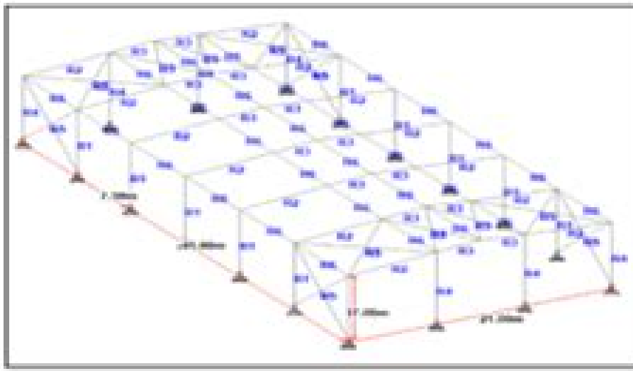
SECTION DIAGRAM FOR INDUSTRIAL WAREHOUSE
