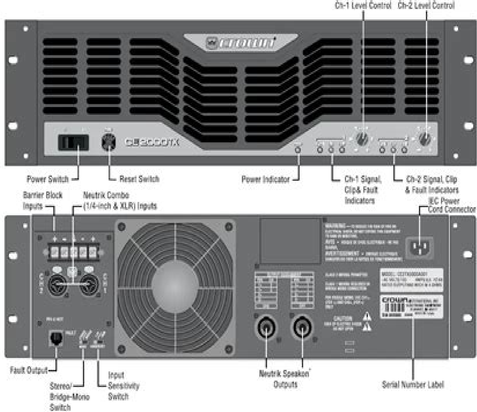
Figure 4.1 Controls, Indicators & Connectors
