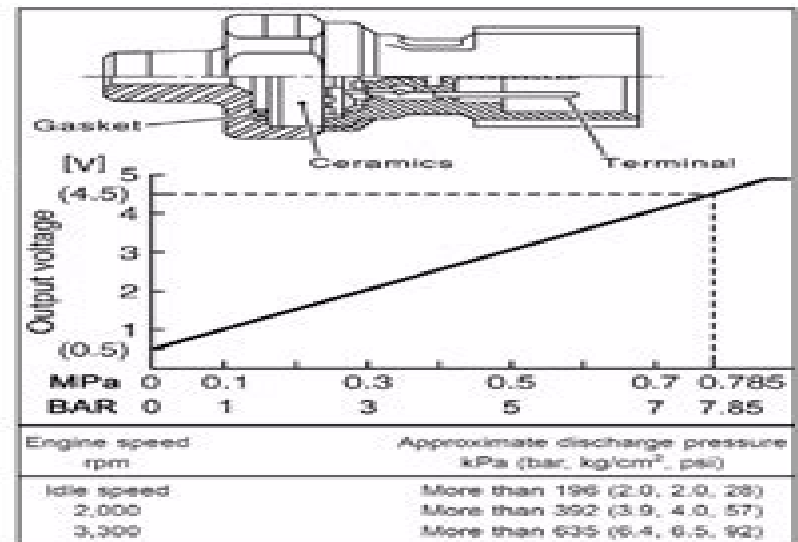
1: Oil Pressure Sensor
