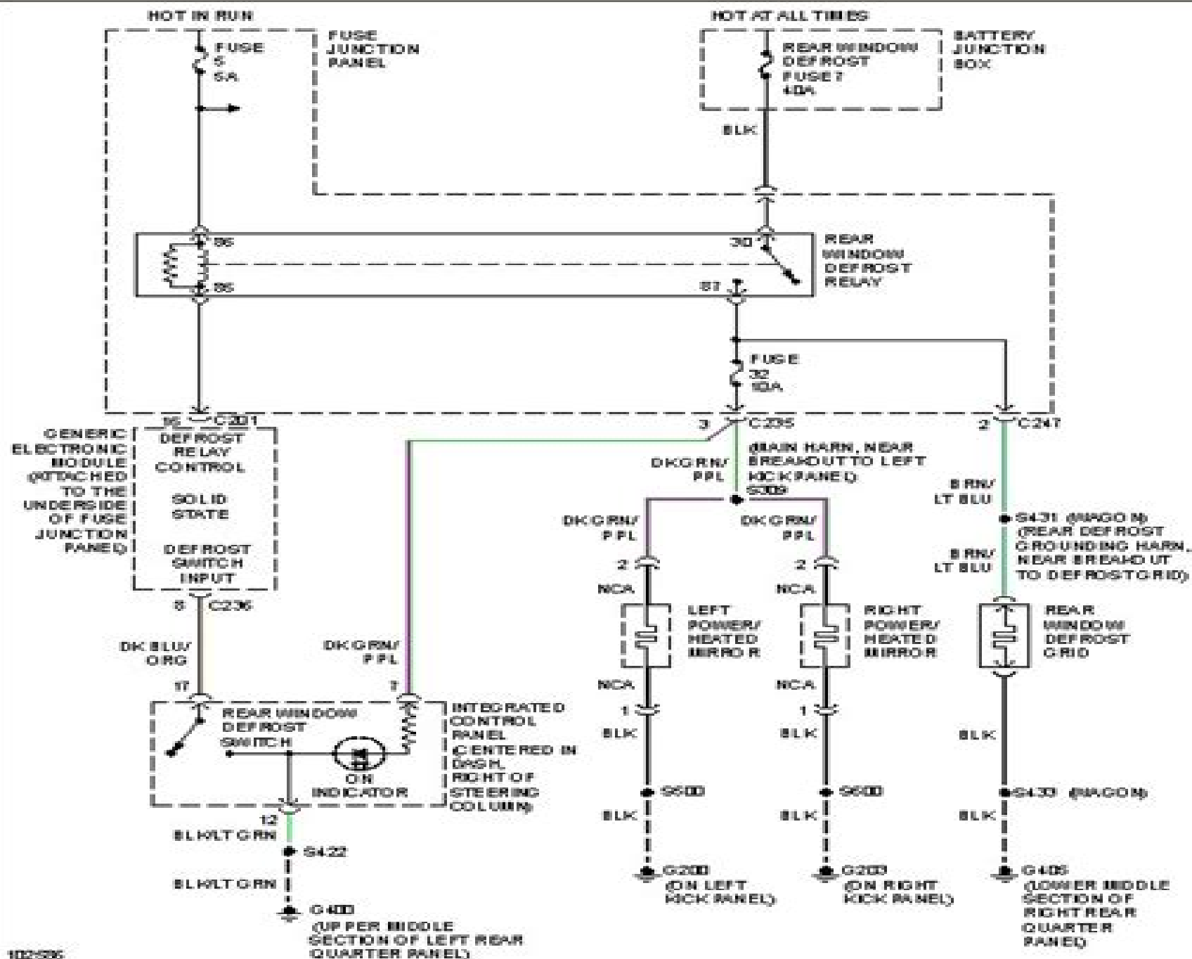
Fig. 11: Defogger Circuit
