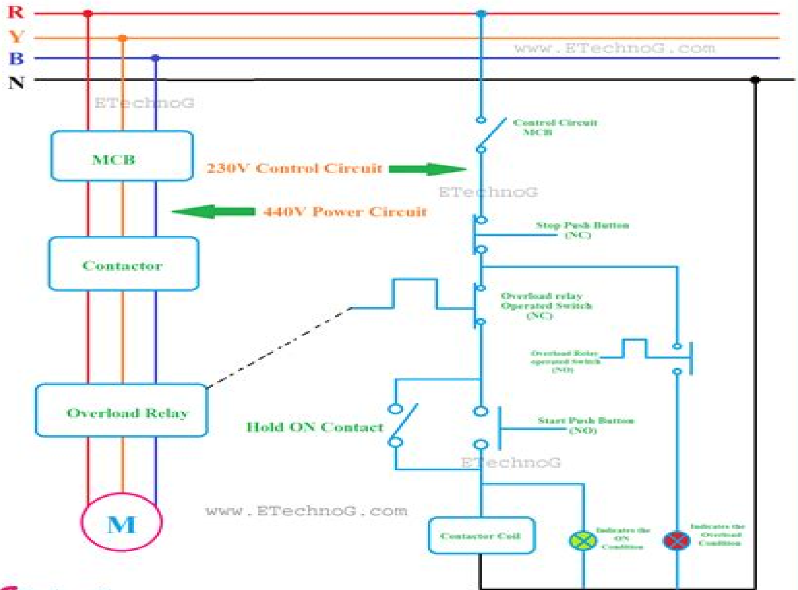
DOL Starter Control Circuit
