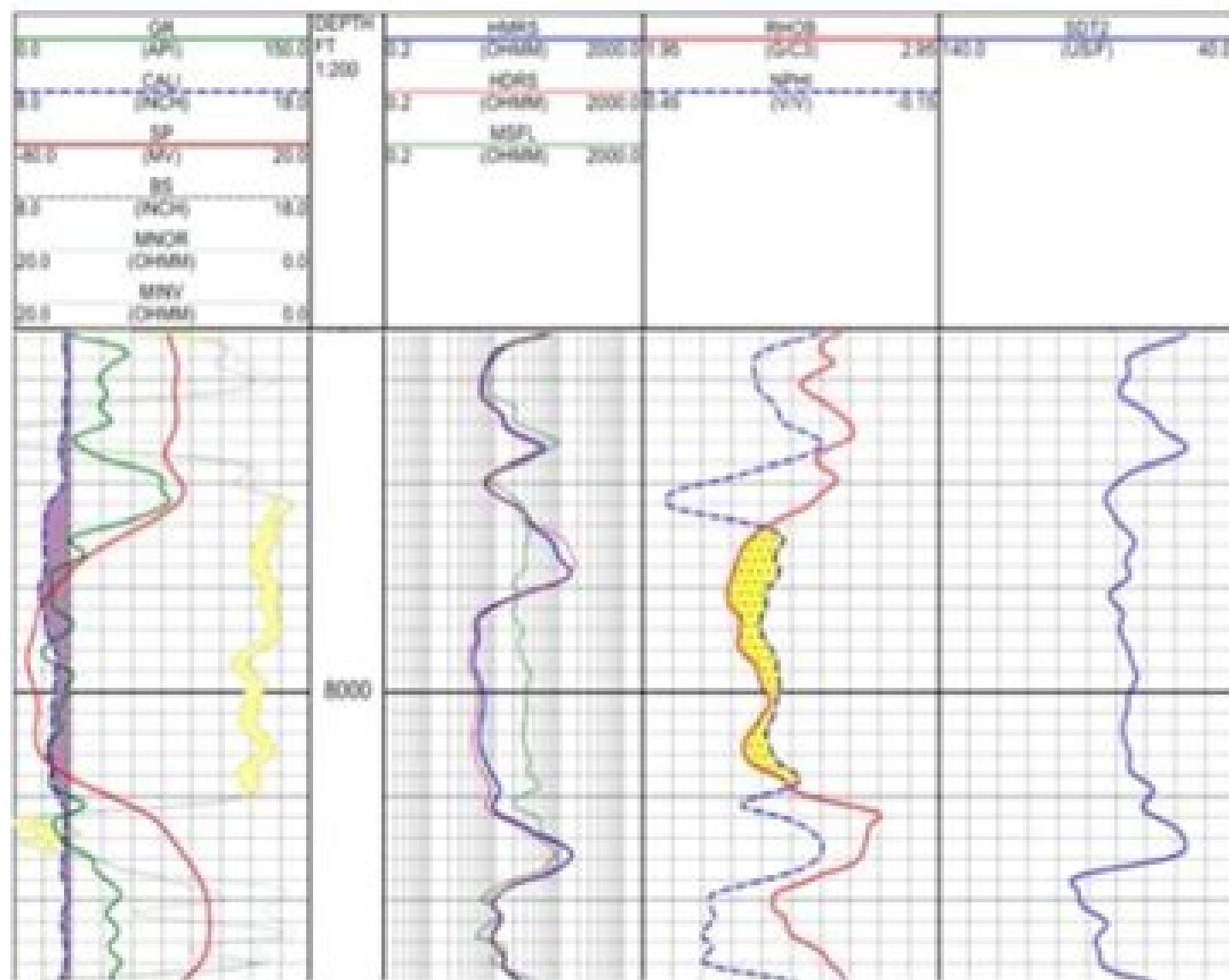
Triple Combo Log Example
