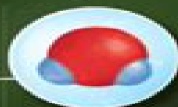
Space-filling model
