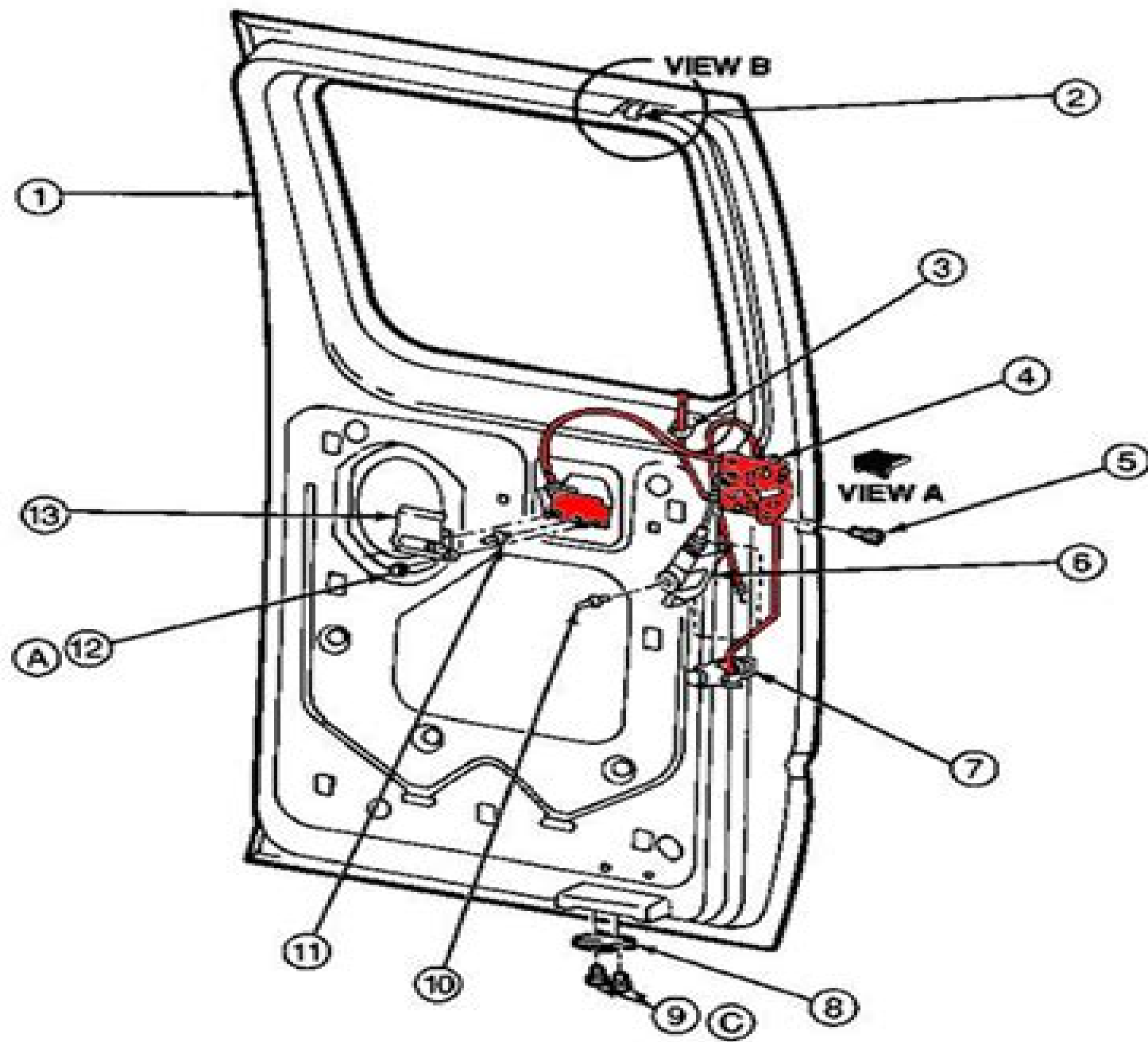
POWER DOOR LOCK SHOWN MANUAL DOOR LOCK TYPICAL
