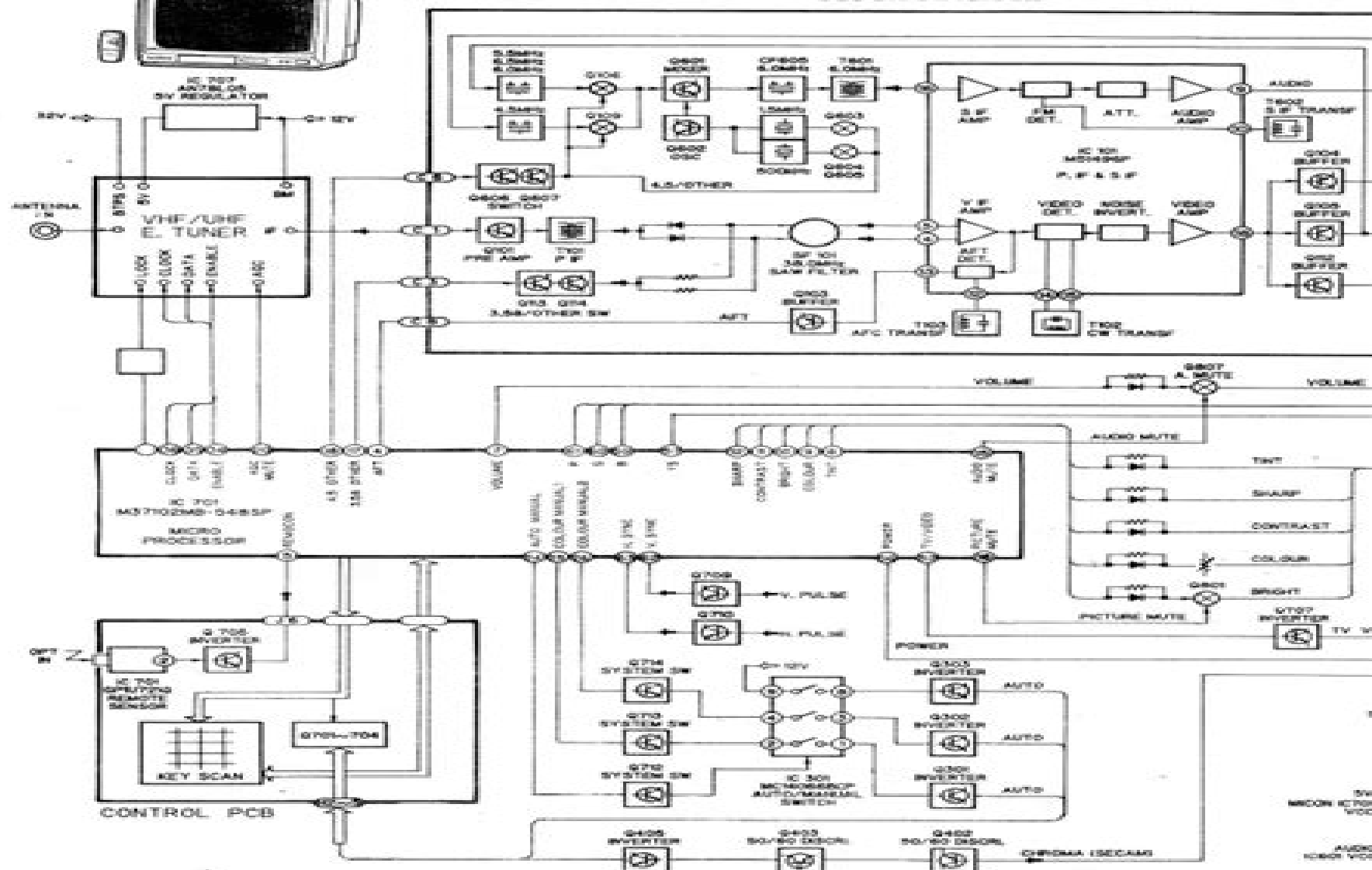
BLOCK DIAGRAM
