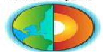
Earth Layers
