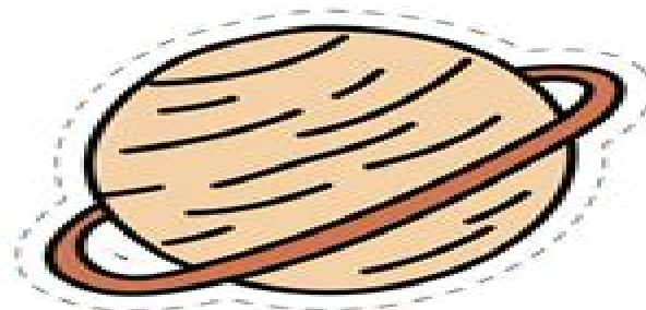
Saturn
