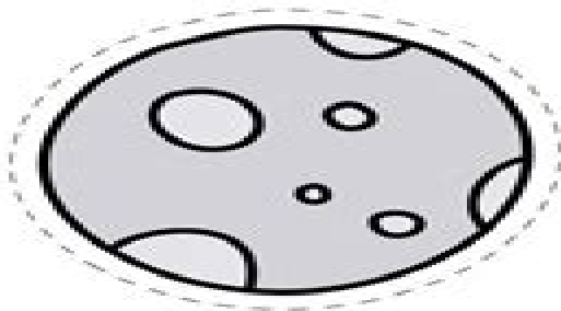
Mercury
