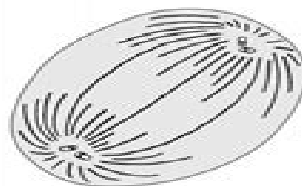
Anaphase II
