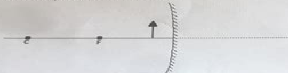
Case 5: Object between F and Mirror
