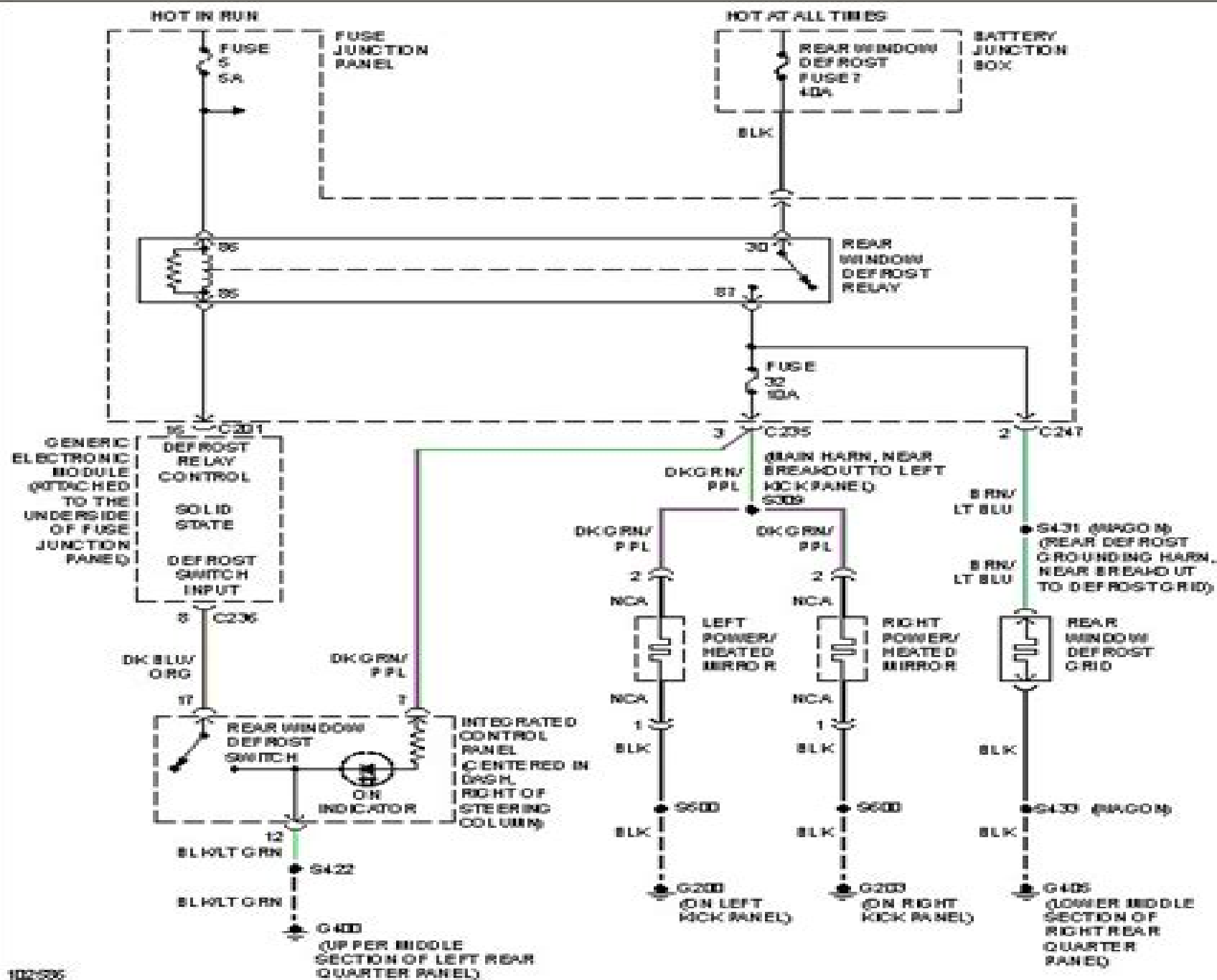
Fig. 11: Defogger Circuit
