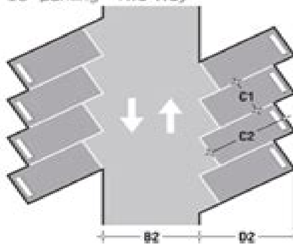
60° parking - Two Way
