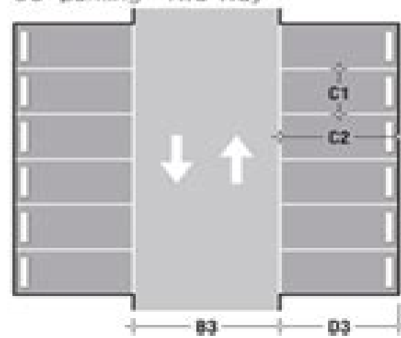
90° parking - Two Way
