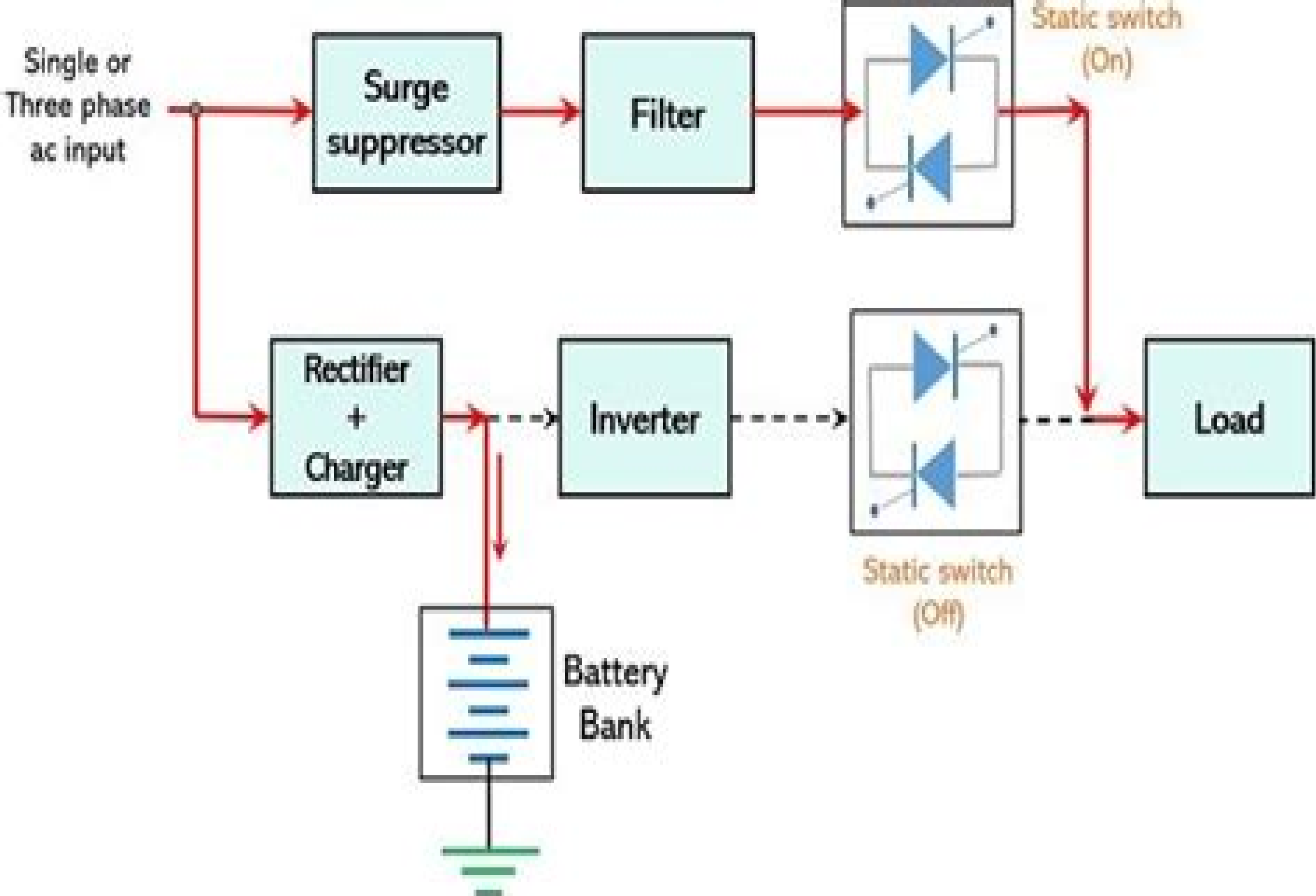
Block Diagram of Off-line UPS System (mains supply on )
