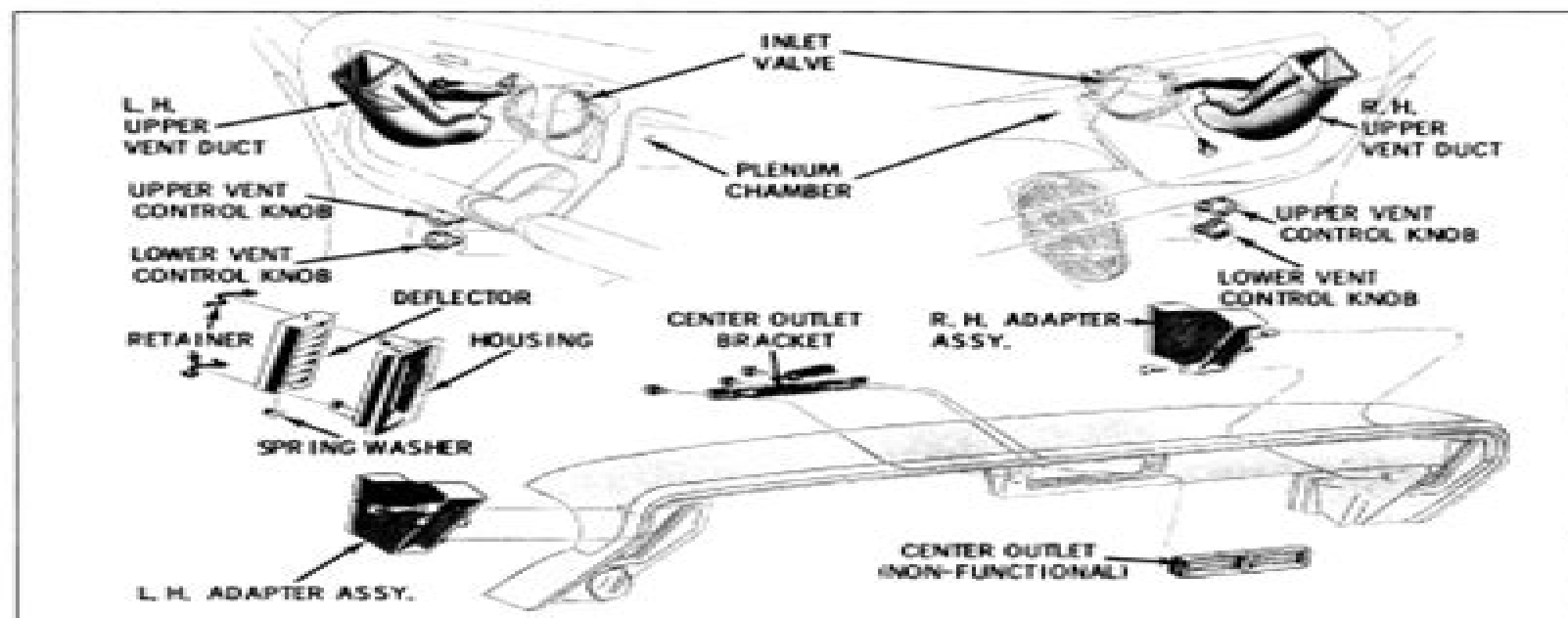
Fig. 1-23—Upper Level Ventilation Outlets
