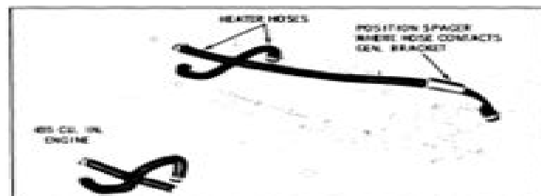
Fig. 1-20—Heater Hose Routing (V-8)
