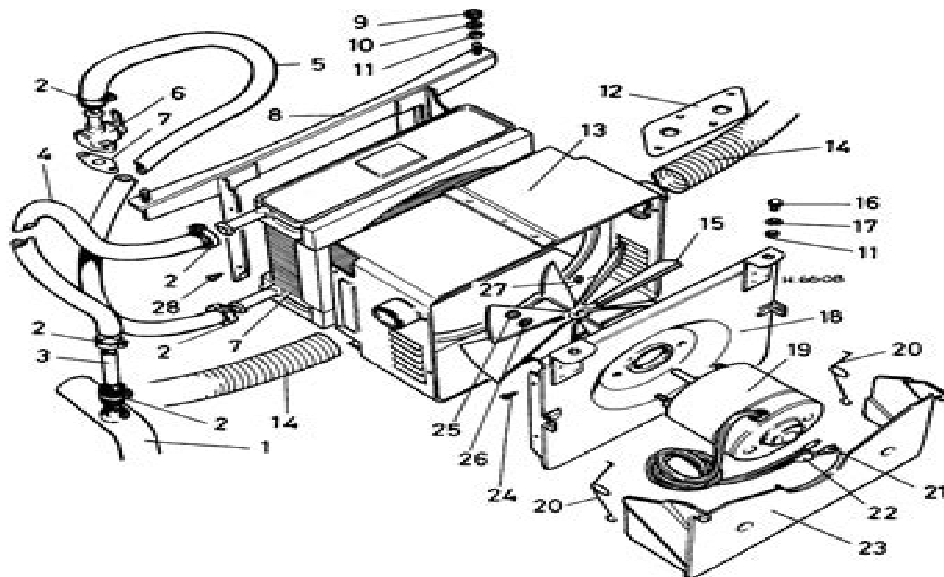
16.2 Exploded view of the recirculatory heater
