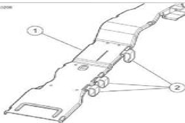
Figure 3-54. Brake Line Retainer
