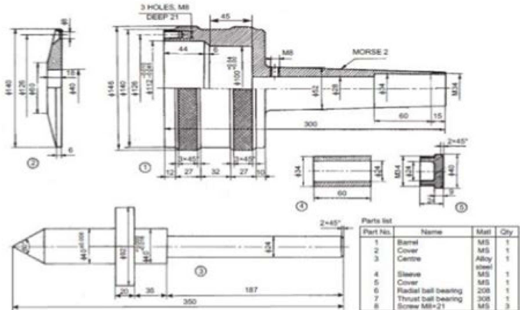
Fig. 18.29 Revolving centre
