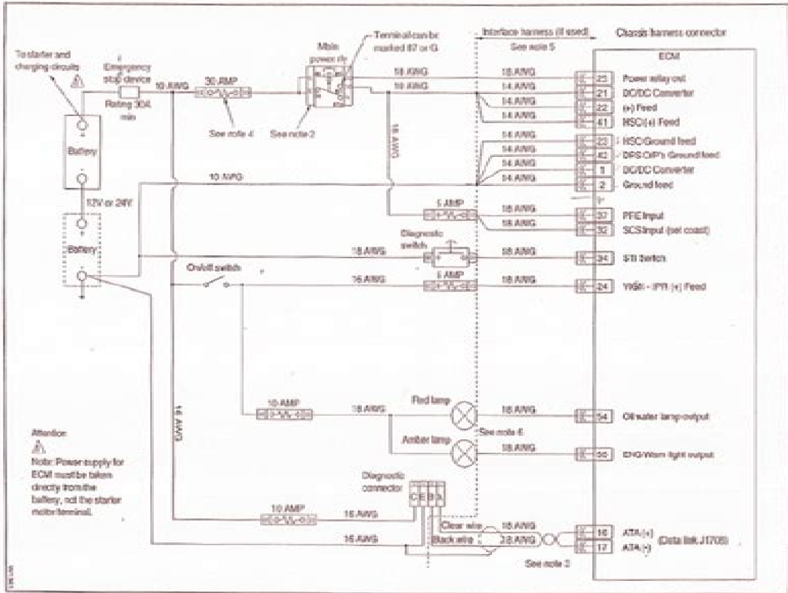
Wiring diagram - Stand alone (asynchronous) running
