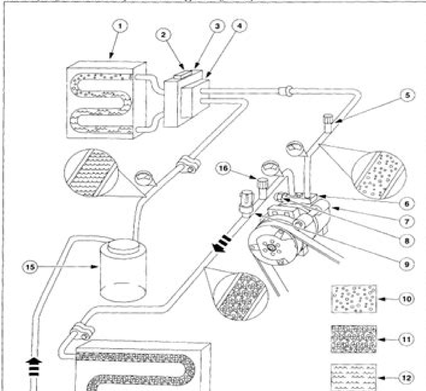
Clutch Cycling Thermostatic Expansion Valve Type Refrigerant System
